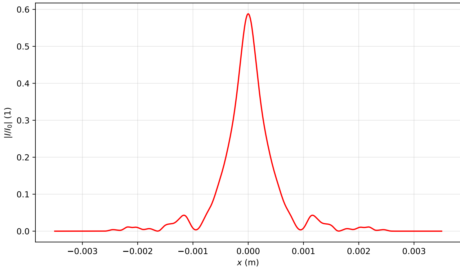
Intensity profile I(x, y = 0, z = 2.388)/I_0 , P_{in}=4.5P_{cr} , artificial time
